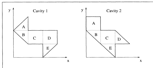
FIG. 1. Geometric shapes of the two two-dimensional domains with identical spectra. The dotted lines are boundary lines dividing the cavities into smaller regions.
